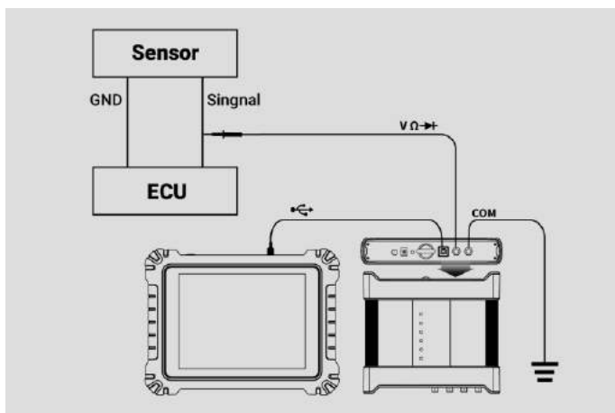
Figure 7-15 Sample Triangle Waveform Connection Diagram
