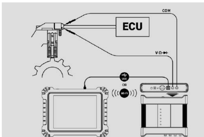
Figure 7-14 Sample Square Wave (X+Y) Connection Diagram
